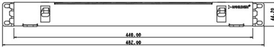
Front View
