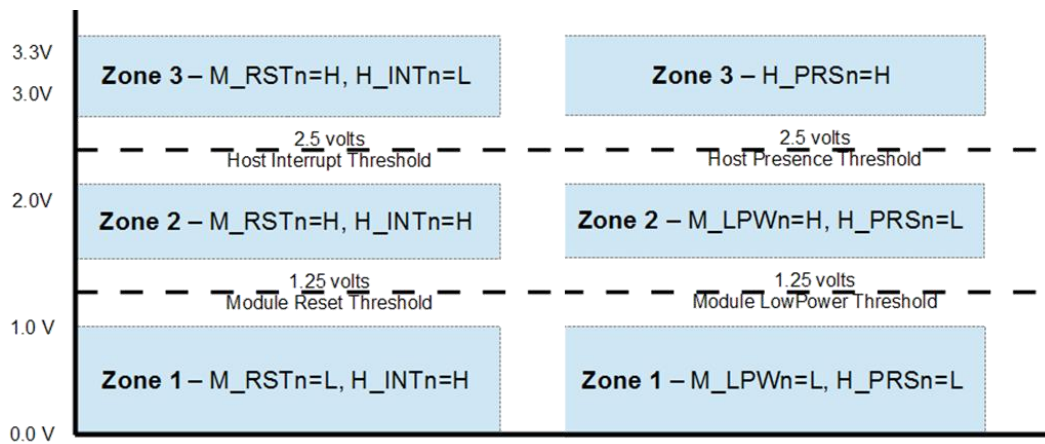
Figure 3. Voltage Zones
