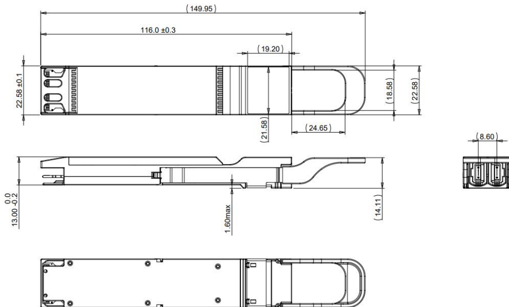
Figure 7. Mechanical Outline (IHS)
