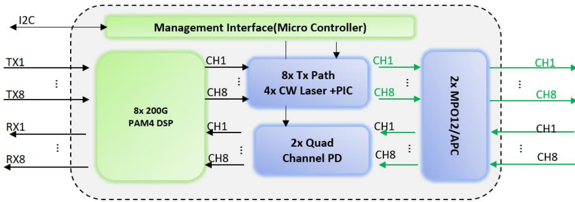
Figure 1. Transceiver Block Diagram
