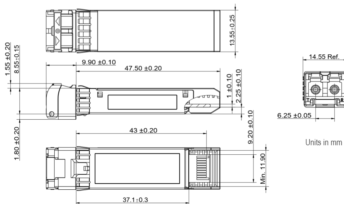
Figure2. Mechanical Outline
