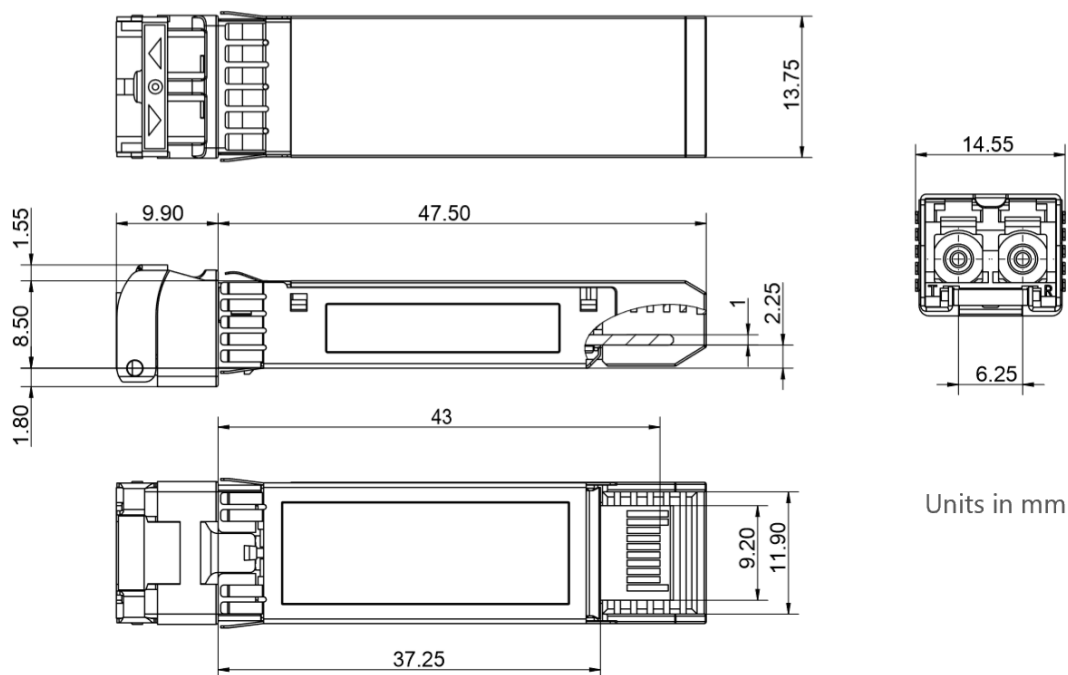
Figure2. Mechanical Outline
