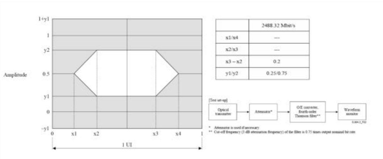
Figure 1 Transmitter Eye Mask Definitions and Test Procedure
