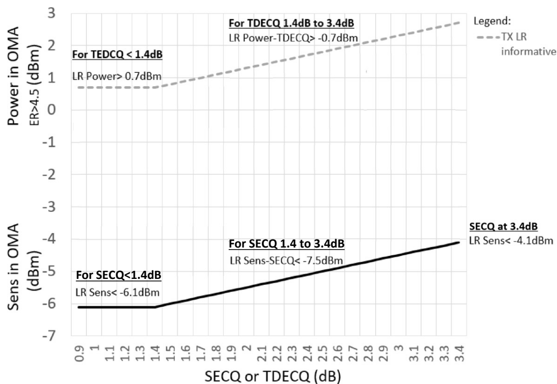
Stressed Receiver Sensitivity Mask for 400G-LR4
