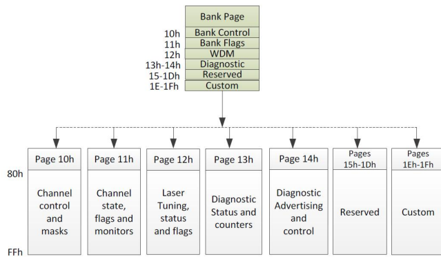
Figure 5.1 CMIS Module Memory Map
