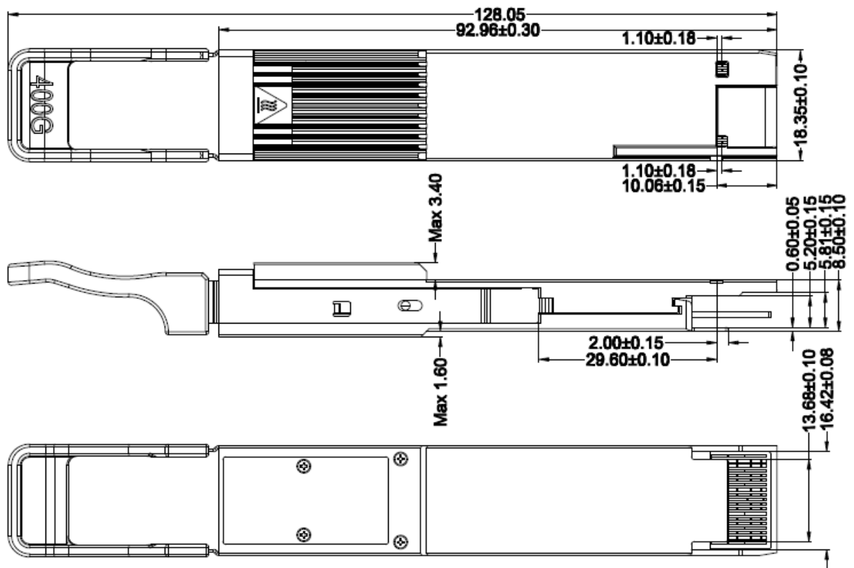
Figure 7.1 Package dimensions
