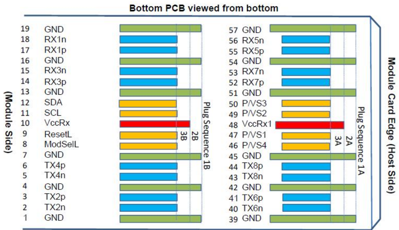
Figure 6.1 QSFP-DD Transceiver Electrical Pad Layout
