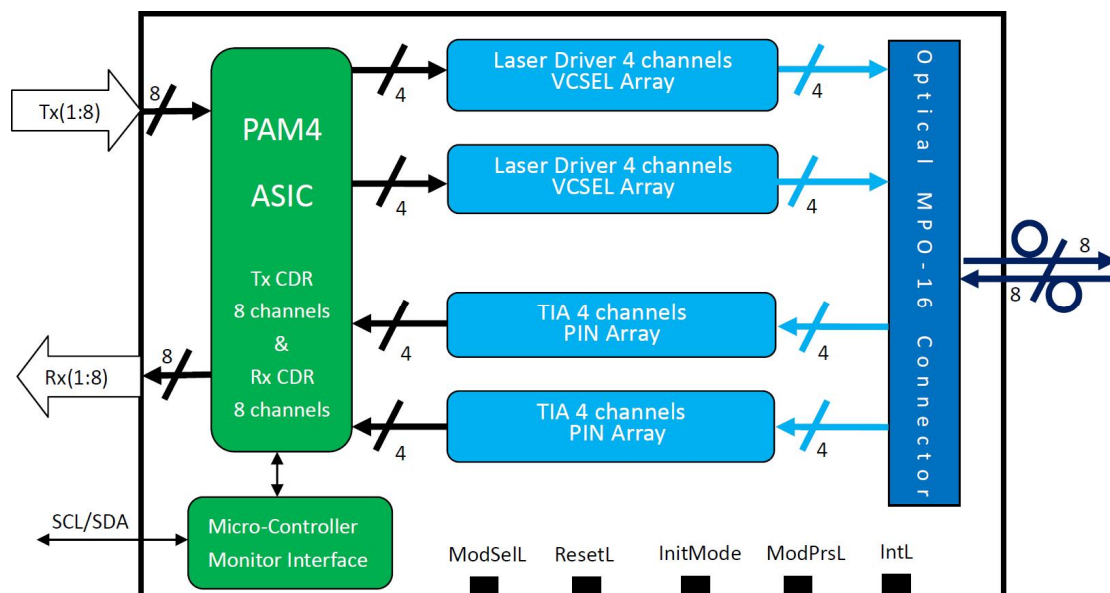
Transceiver Block Diagram
