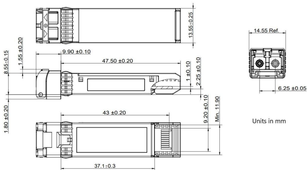
Figure2. Mechanical Outline
