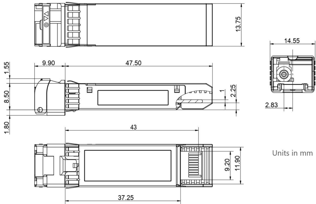
Figure2. Mechanical Outline
