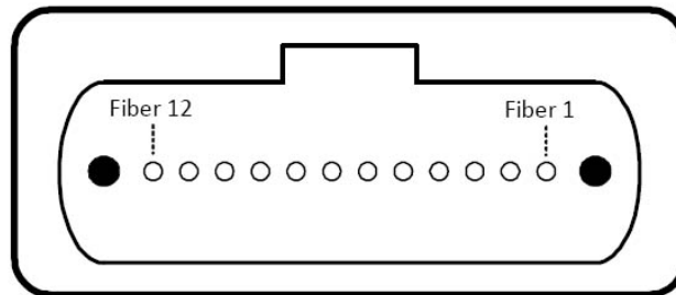
Outside View of the QSFP Module MPO
