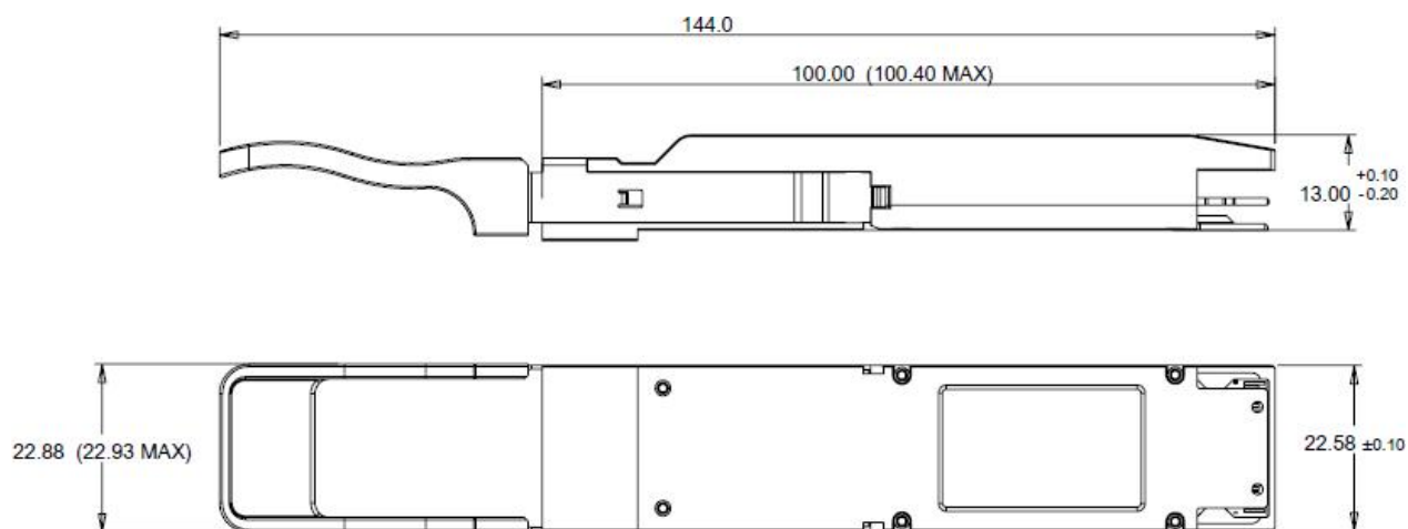
Figure 5. Mechanical Outline
