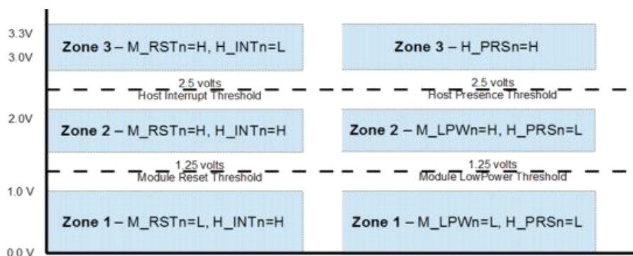
Figure 1. Voltage Zones
