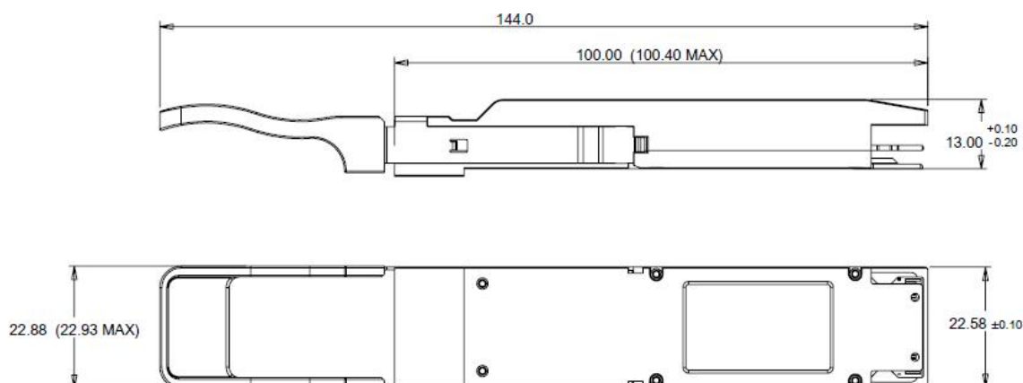
Figure 6. Mechanical Outline
