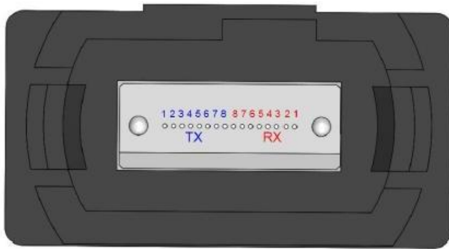
Figure 4. MPO-16 Optical Connector Interface
