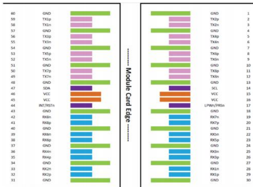
Figure 3. MSA Compliant Connector
