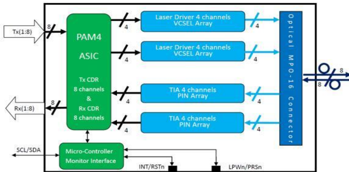
Figure 2. Transceiver Block Diagram
