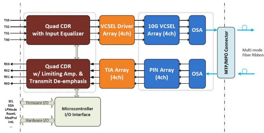
Figure1: Block Diagram
