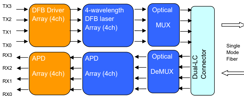
Figure 1: 40Gb/s QSFP ZR4 Transceiver Block Diagram
