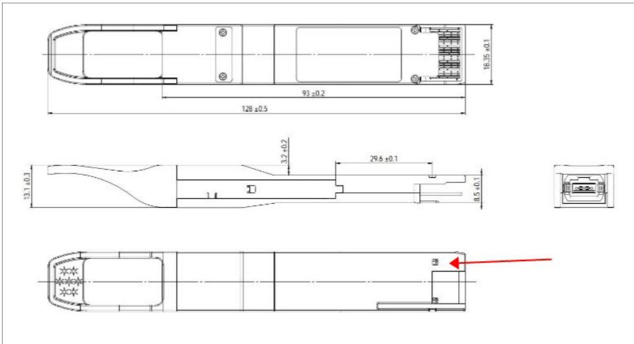
Figure10. Mechanical Specifications
