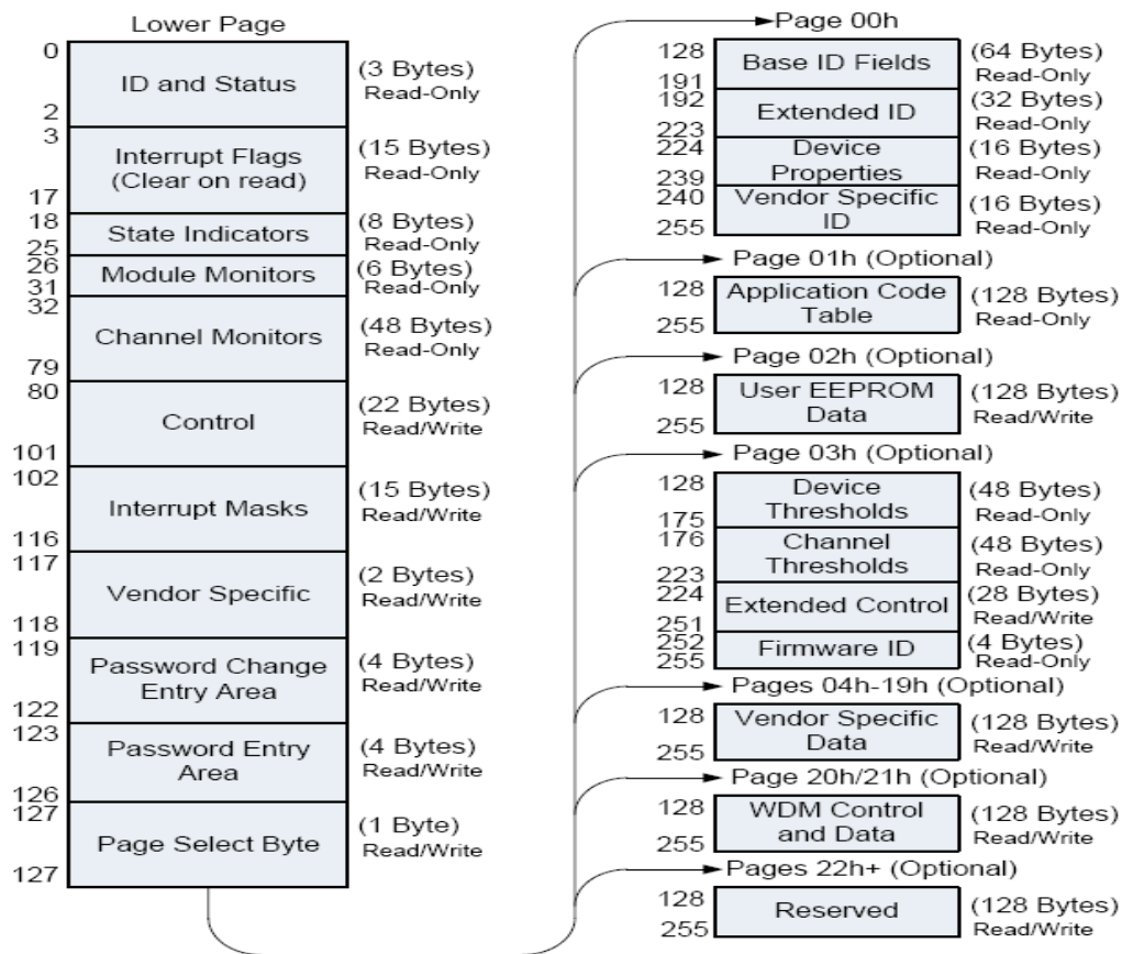
Figure 5. QSFP28 Memory Map
