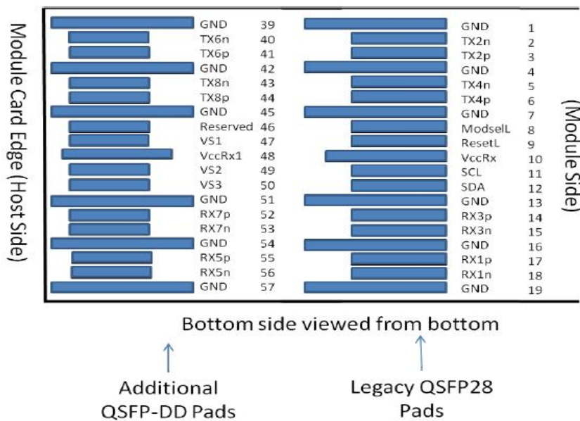
Figure 2. Electrical Pin-out Details
