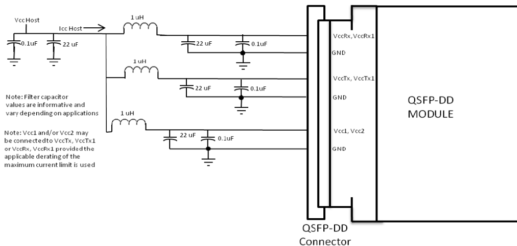
Figure 3. Host Board Power Supply Filtering
