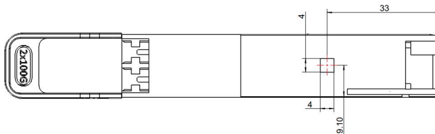
Figure 9: Case Temperature Measurement Point (All dimensions in mm)
