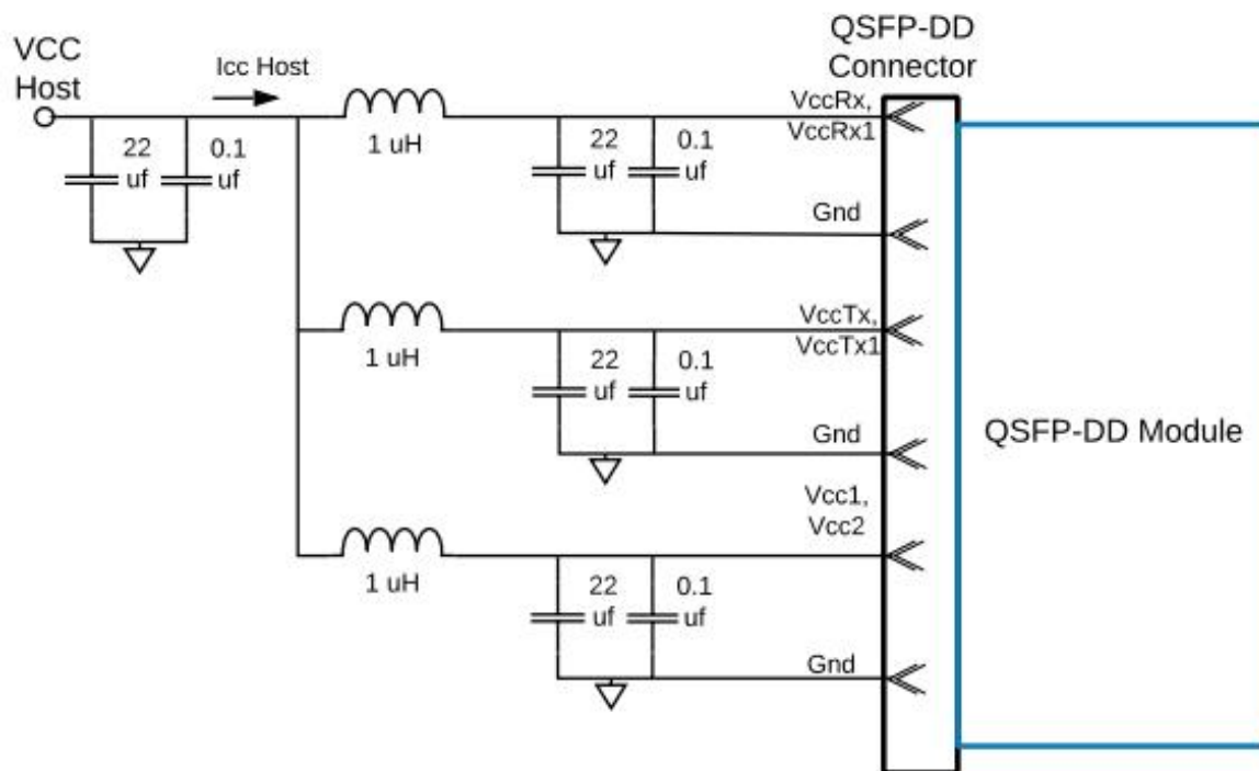
Figure 7: Host Board Power Supply Filter
