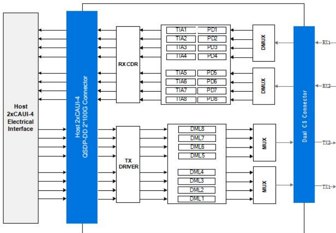
Figure 2: Application Reference Diagram
